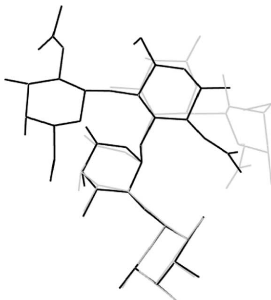
Figure 2. Overlay of modeled structures of FFFGn (gray) and LDNDF (black). The Fuc \alpha 1-2Fuc Moiety of LDNDF overlays almost perfectly with the terminal Fuc \alpha 1-2Fuc moiety of FFFGn, this might be the explanation for the binding of Mab 114-5B1-A to both these structures. The picture was created using PyMol Molecular Graphics System (DeLano, W.L. 2002, http://www.pymol.org ).
