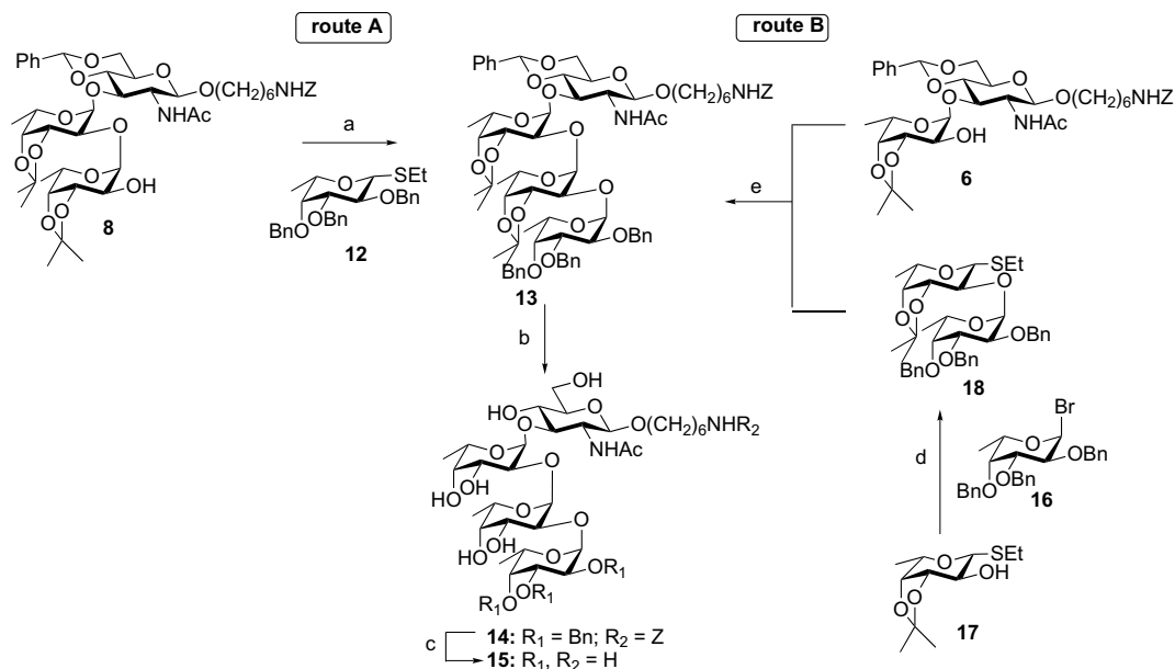
Scheme 2. Reagents and conditions: a. CuBr 2 , Bu 4 NBr, DMF–CH 2 Cl 2 (1:1), 16%. b. HOAc 60%, 50 °C, 57%. c. H 2 , Pd/C, EtOH, HCl 1 M, 70%. d. (1) 12 , Br 2 , CH 2 Cl 2 , 0 °C; (2) Bu 4 NBr, DMF–CH 2 Cl 2 , rt, 68%. e. CuBr 2 , Bu 4 NBr, DMF–CH 2 Cl 2 (1:1), 52% (α/β 2.3:1).
